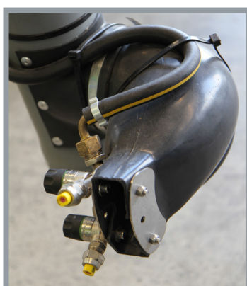
OUTLET & NOZZLES
